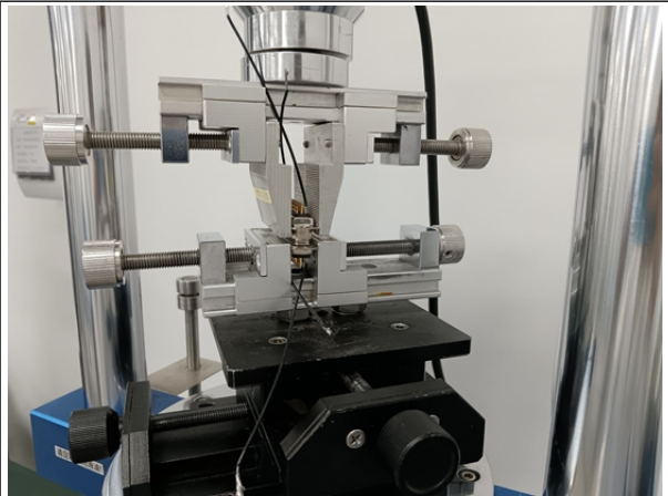
During Test-Sample A- Mating Cycle Testing
