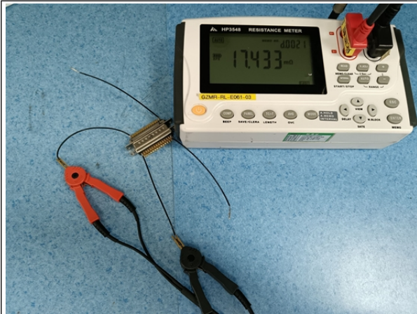
During Test-Sample A- Contact resistance
